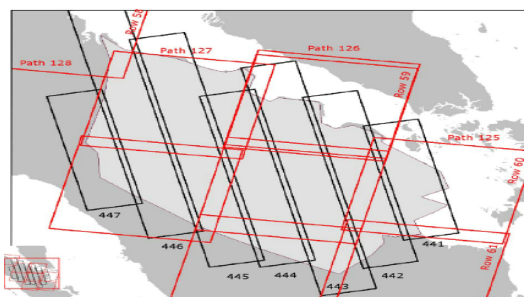
Figure 1 : Illustration of the different acquisitions used in this study with their corresponding footprint in Riau: PALSAR strips in black and Landsat scenes used for the WWF land cover classification in red.
