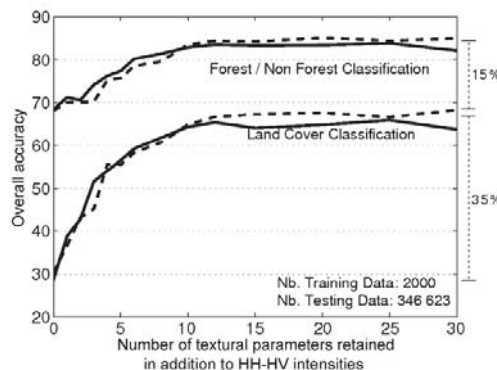
Figure 3 : Accuracy of the SVM-based classification at local scale depending on the number of textural parameters used as input in addition to the HH/HV channels.
