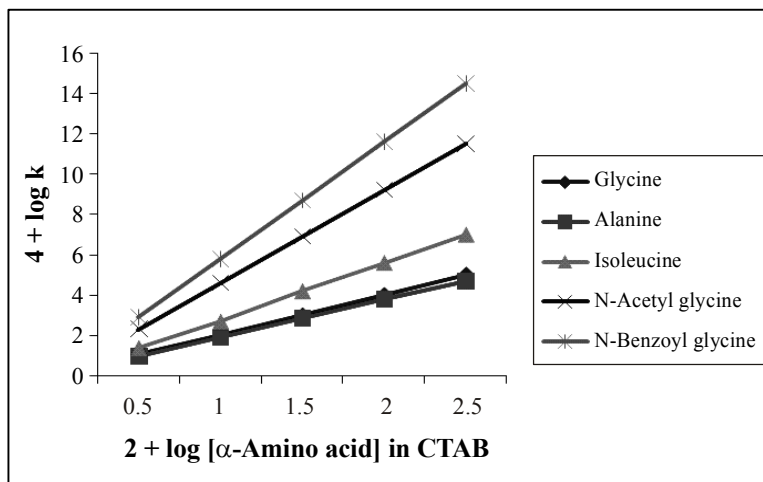
Fig. 1: Dependence of rate on [\alpha\text{-Amino acid}] in NaLS
