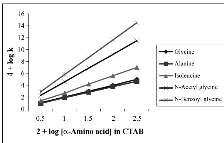
Fig. 2: Dependence of rate on [\alpha\text{-Amino acid}] in CTAB
